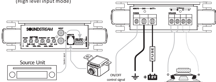
Fig 12. Mono amplifier wiring (High level input mode)
