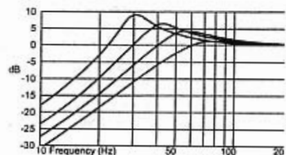
FIG. 6 VARIOUS SETTINGS
