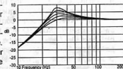
FIG. 2 VARIABLE BOOST
