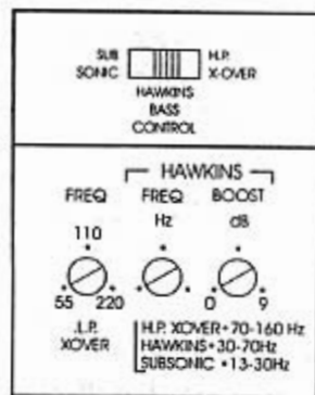
FIG. 1 BASS CONTROL
