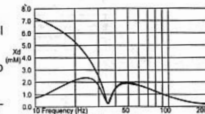
FIG. 3 Limited Excursion
