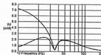
FIG. 5 LIMITED EXCURSION
